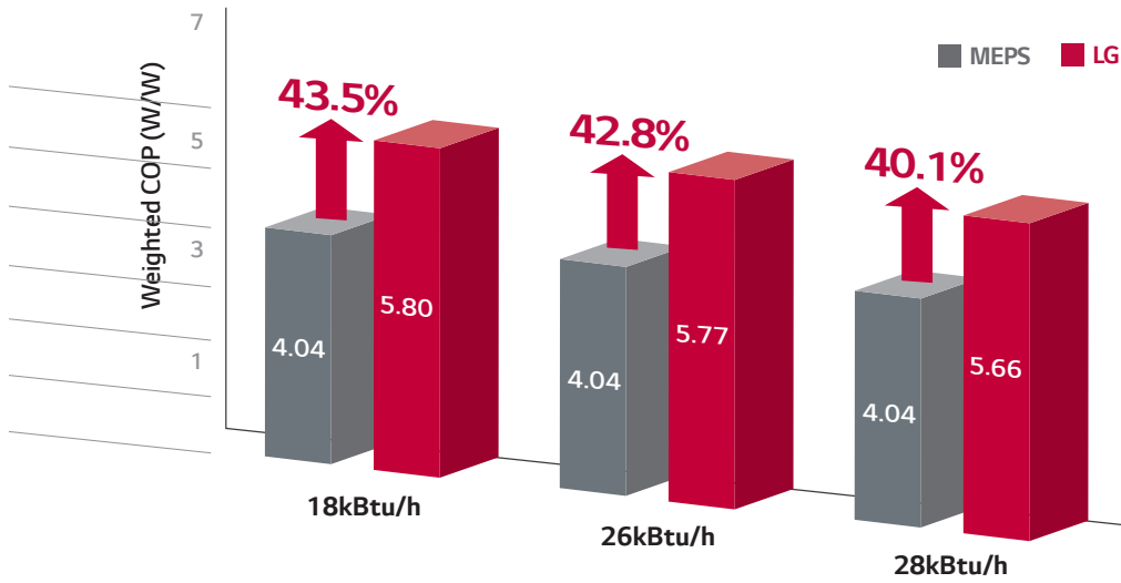
Weighted COP Comparison (LG vs MEPS)
